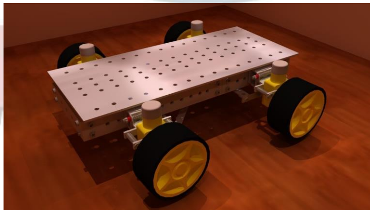
Fig 5.2.3 Chassis
